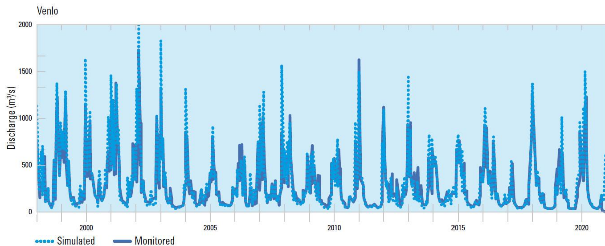
Figure 61 Simulated and monitored decade flows at gauging station Venlo (Netherlands) from 1998 to 2020.
